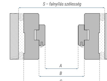
Dimensions of Std 2-pack door frame [mm]:
